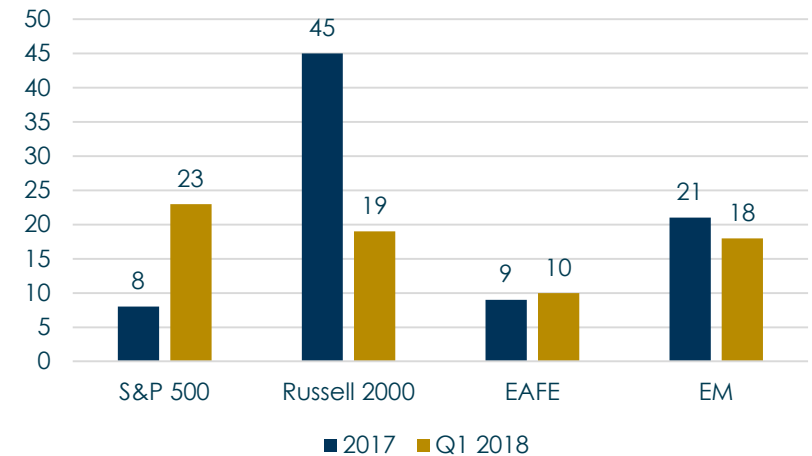
Count of Days with Daily Return Larger than +/- 1% Magnitude
